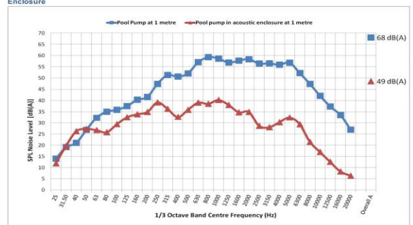
Figure 6.1 Overall A-Weighted & 1/3 Octave Band Noise Levels - Pool Pump With and Without Acoustic Enclosure
